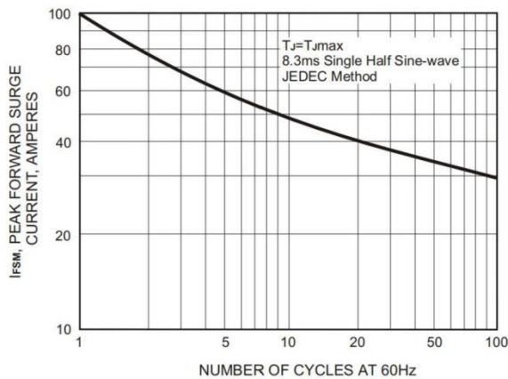
Figure5. Maximum Non-Repetitive Forward Surge Current Uni-Directional Only
