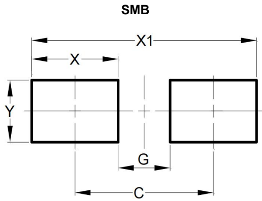
Fig. Soldering footprint for SMB
